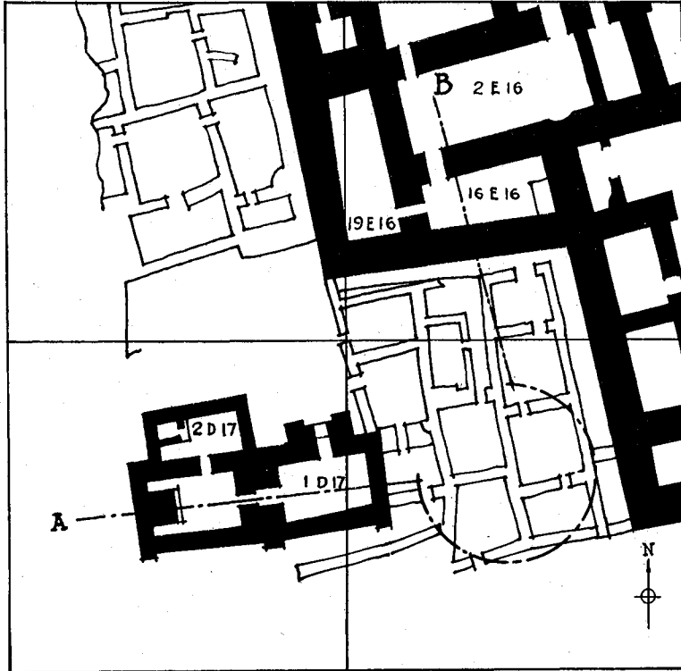
FIG. 89.—Key plan showing location of section through temple of Abu and palace at Tell Asmar as given in folding plate at end. Scale, 1:400.
