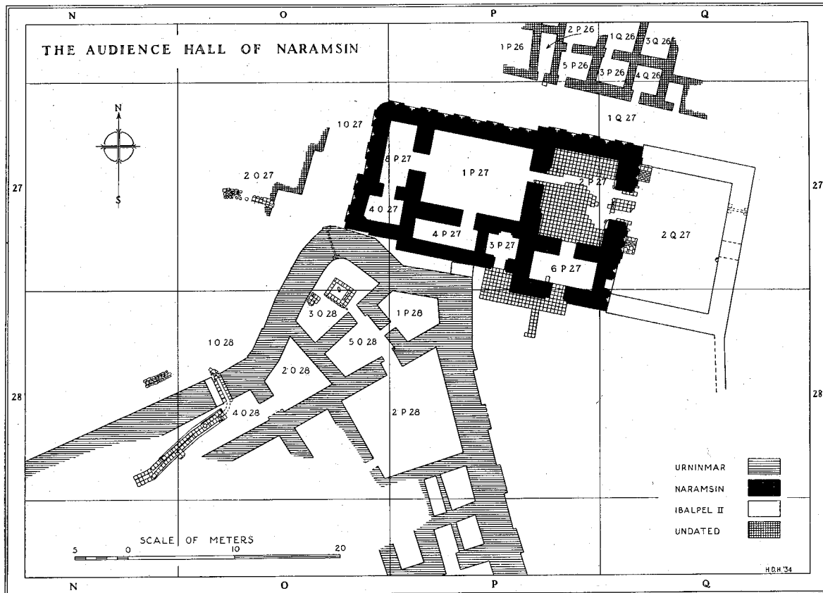
FIG. 3.—Plan of the audience hall of Naramsin and adjacent structures at Tell Asmar. Scale, 1:500
