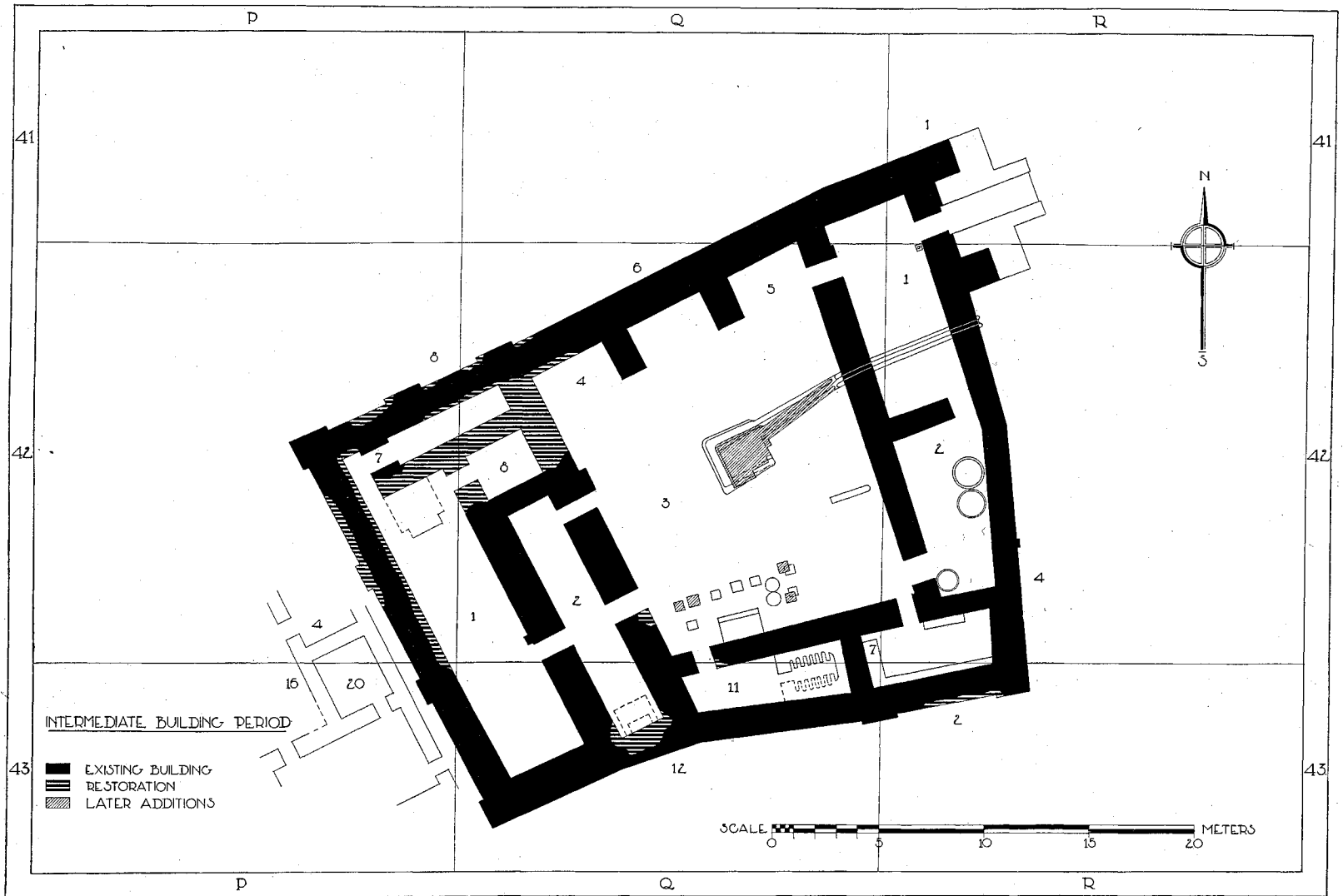
FIG. 45.—The temple of Sin. Plan of the intermediate building level. Scale, 1:300
