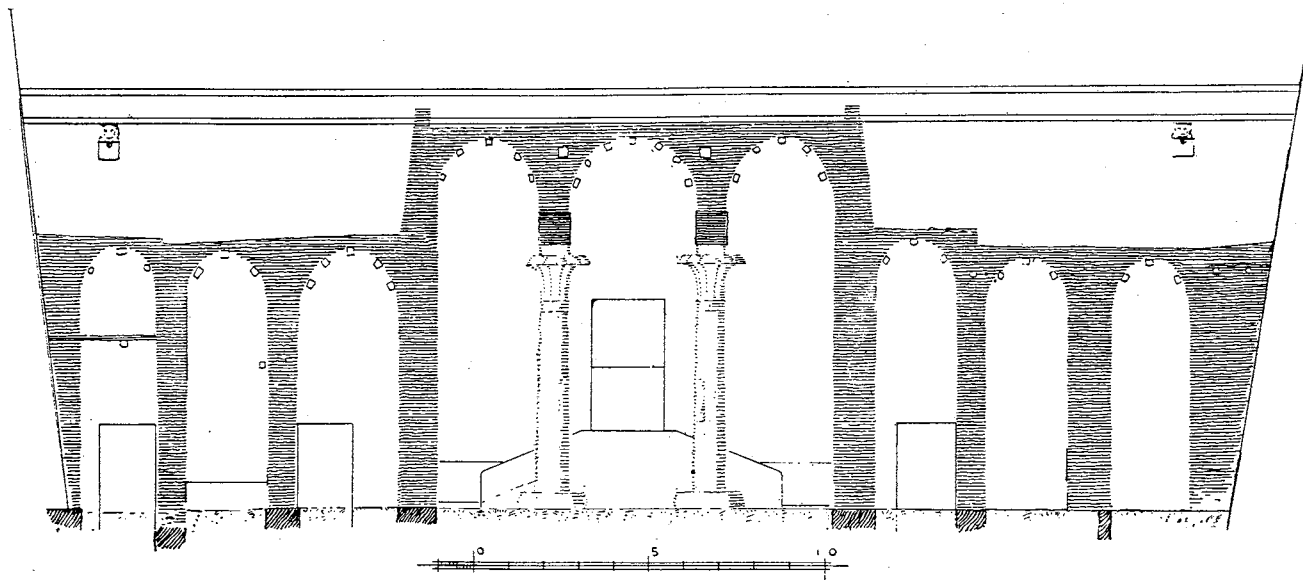
FIG. 35.—CROSS-SECTION THROUGH THE AUDIENCE HALL OF THE SECOND PALACE OF RAMSES III AT MEDINET HABU
