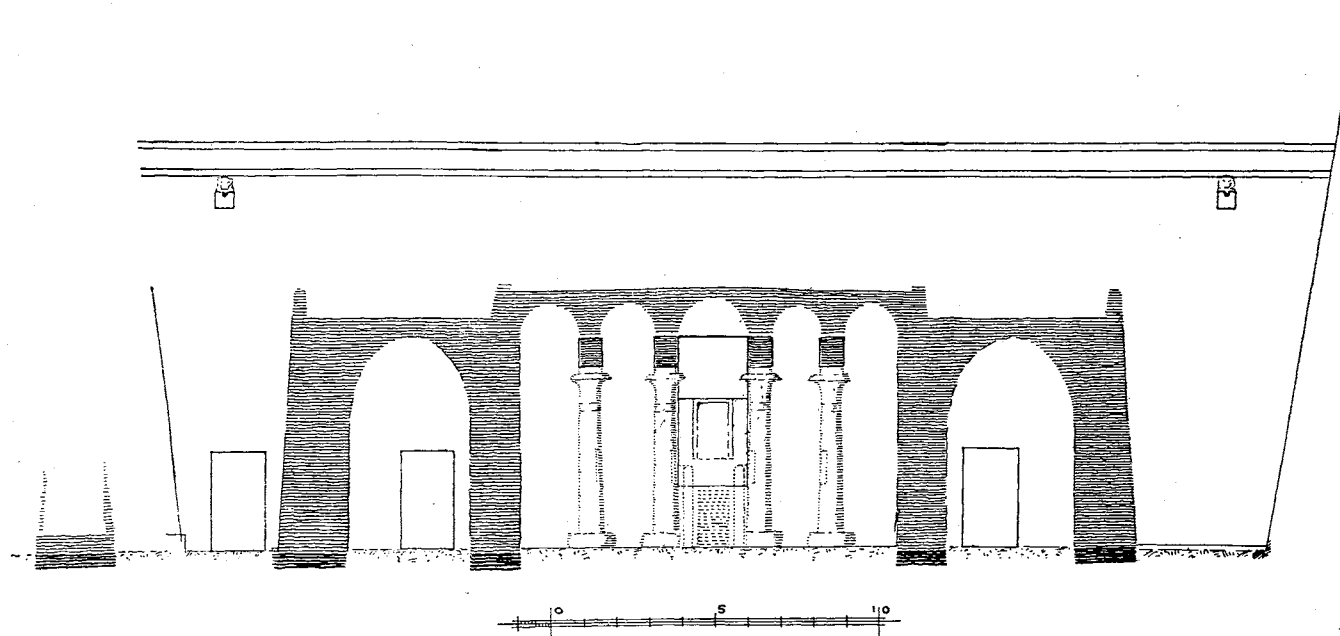
FIG. 34.—CROSS-SECTION THROUGH THE AUDIENCE HALL OF THE FIRST PALACE OF RAMSES III AT MEDINET HABU
