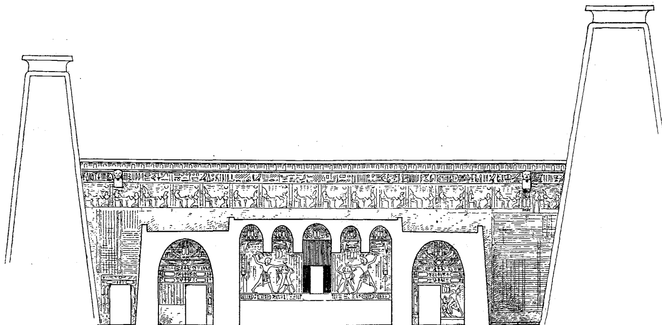
FIG. 33.—REAR ELEVATION OF THE FRONT WALL OF THE PALACE, SHOWING ALSO THE DISPOSITION OF THE BRICK WALLS AND ROOF OF THE FIRST PALACE AT THE POINTS OF CONTACT WITH THE STONE MASONRY FRONT WALL.
